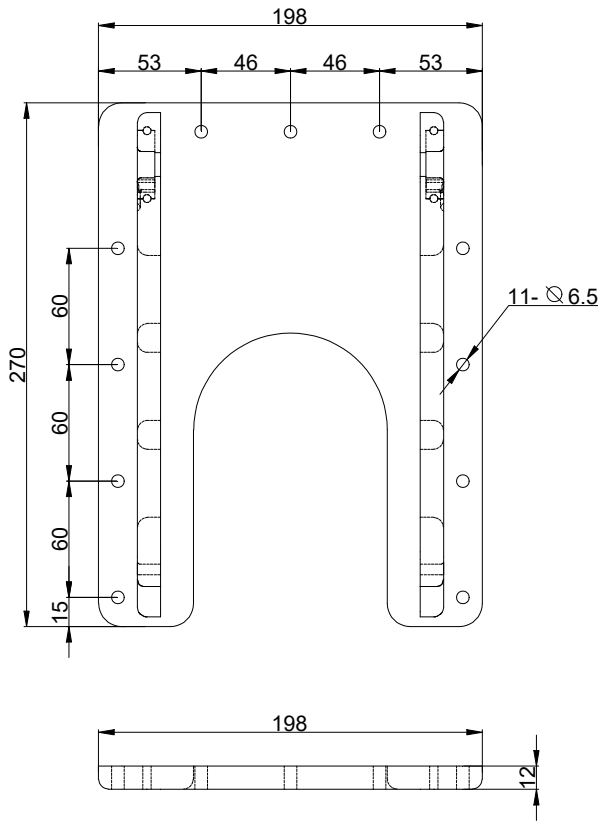
SS90 Standart Taban
