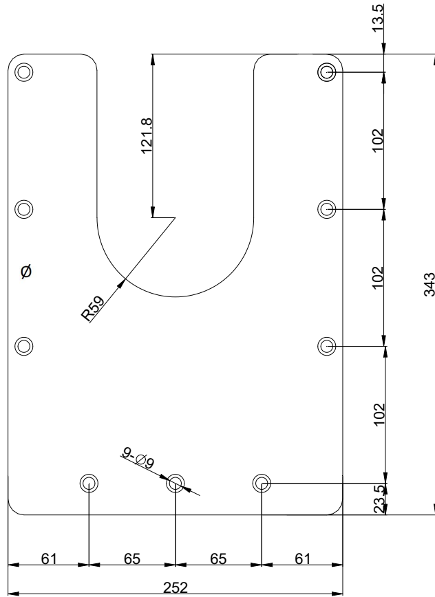
SS180 Standart Taban
