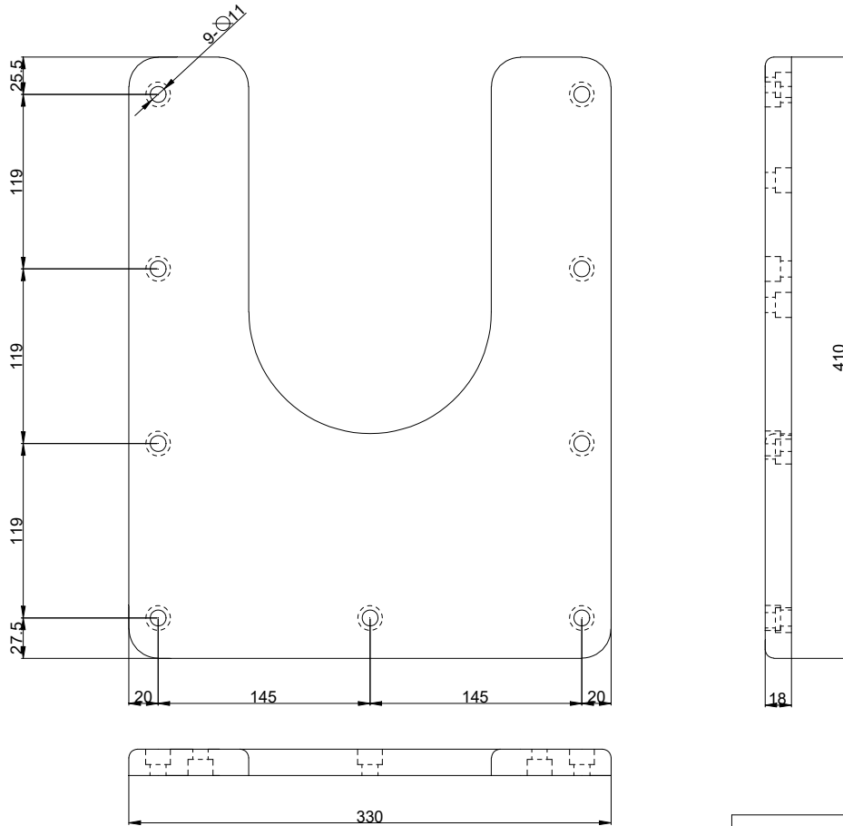
SS280 Standart Taban
